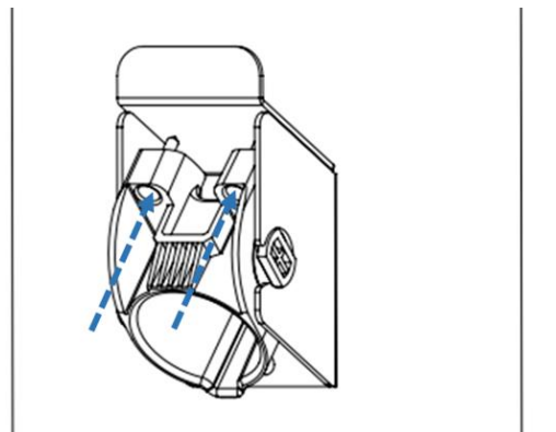
Figure 2-22 Lock screws
