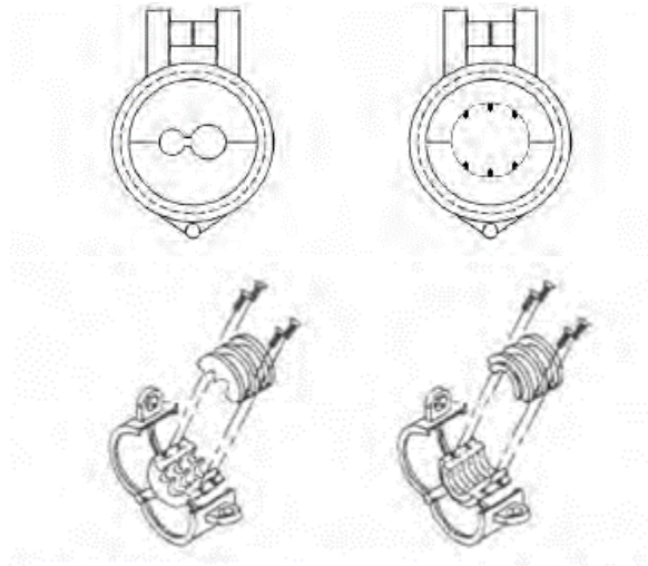
Figure 2-2 Cable Clamp installation
