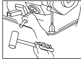
Figure 1 – Remove Core Plug
